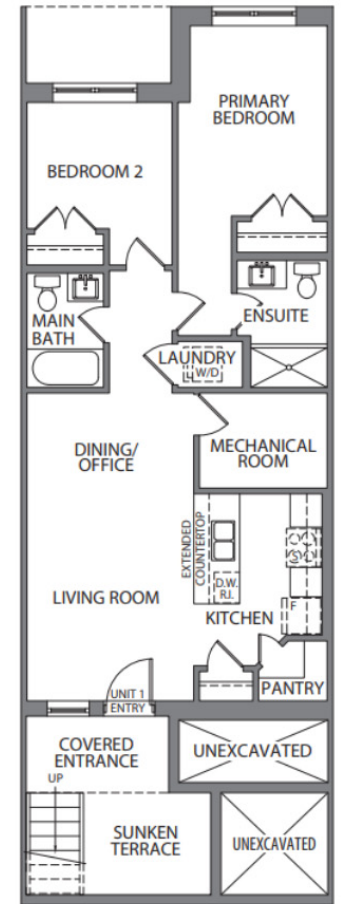
TERRACE LEVEL FLOOR PLAN
